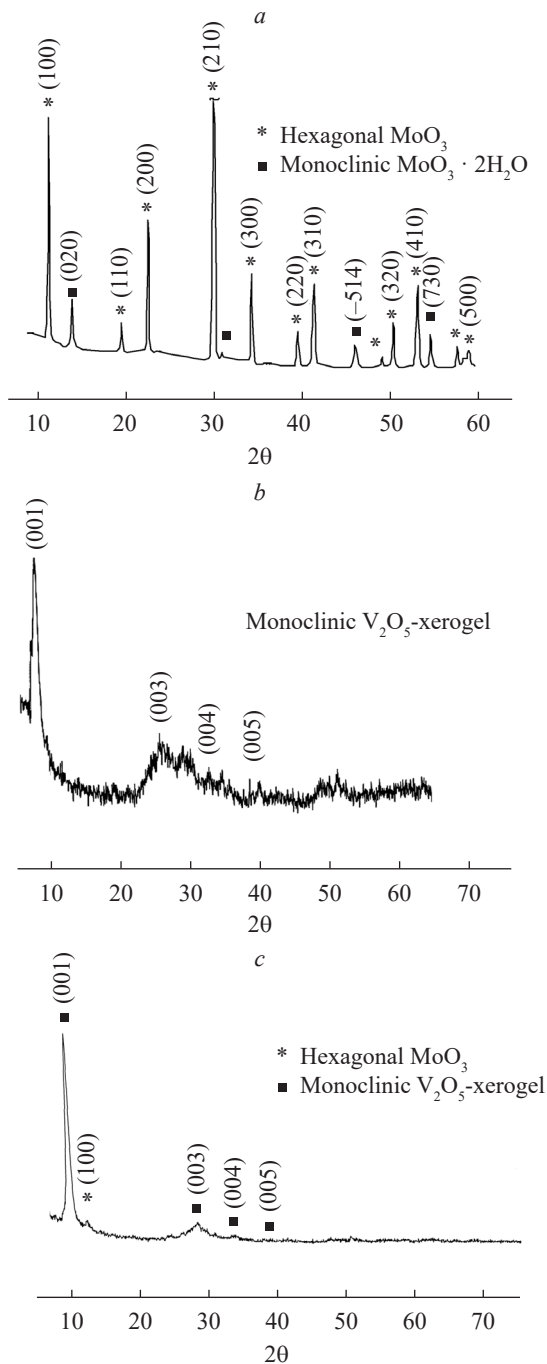
Fig. 1. XRD patterns of \text{MoO}_3 (a), \text{V}_2\text{O}_5 (b) and \text{V}_2\text{O}_5 : \text{MoO}_3 (c)
