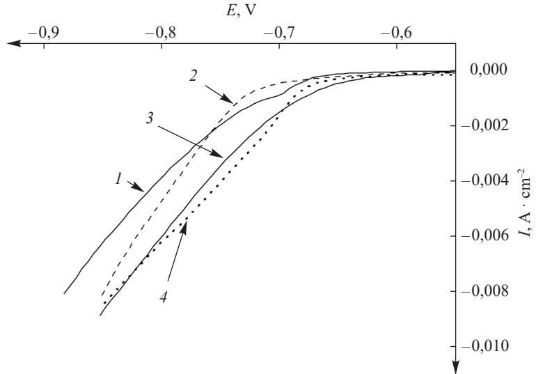
Fig. 4. Potential-current curves for electrochemical deposition of nickel (1) and Ni-MoO 3 (2), Ni-V 2 O 5 (3), Ni-MoO 3 : V 2 O 5 (4) composites
