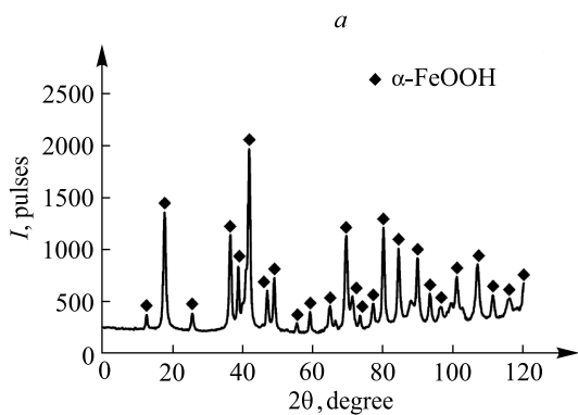
Fig. 1. XRD pattern ( a ) and SEM image ( b ) of the sample of \alpha -FeOOH NP
