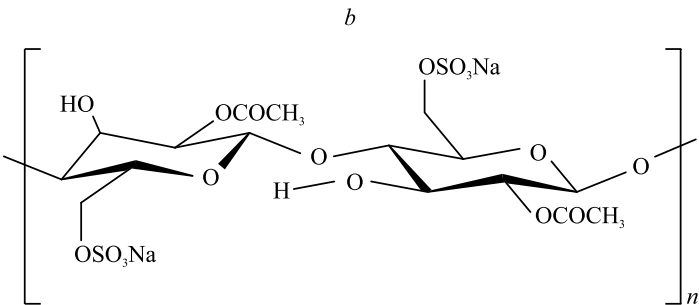
Fig. 1. Structural formulas of KAN ( a ) and Na-CAS repeated unit ( b )
