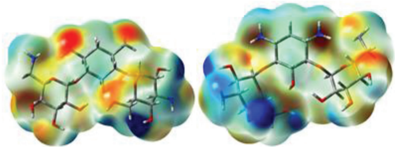
Fig. 14. MEP mapped on a SCF density of KAN monomer
