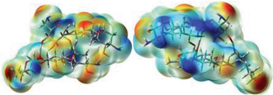
Fig. 15. MEP mapped on a SCF density of KAN A dimer
