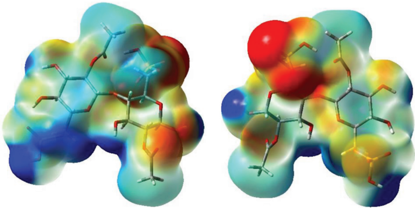
Fig. 16. MEP mapped on a SCF density of CAS (cellobiose fragment)
