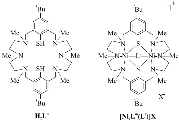
Fig. 1. Structure of Robson-type ligand H_2L^m and its complexes [Ni_2L^m(L^c)]X : X – anion, L^c – coligands
