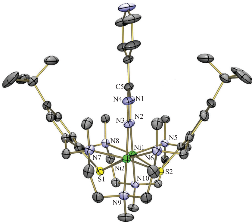
Fig. 4. ORTEP representation of the structure of [\text{Ni}_2\text{L}^{\text{m}}(\text{PyrCN}_4)]^+ . Ellipsoids are represented at 50 % probability. H atoms were omitted for clarity
