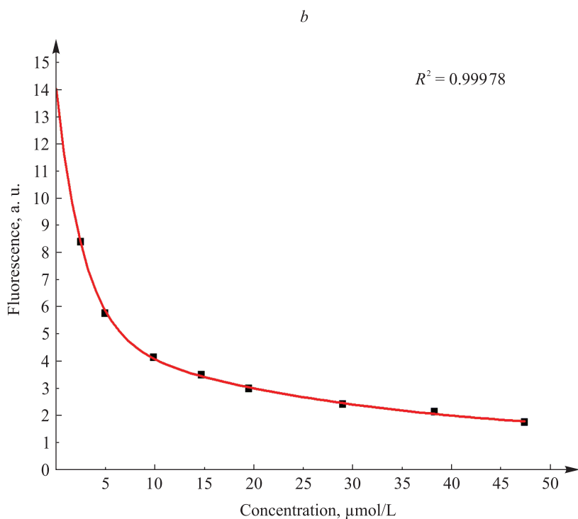
Fig. 3. Decrease of BSA (1 \mu\text{mol/L} ) intrinsic fluorescence (excitation at 295 nm, depicted by dashed line) during direct titration by 4 (2.5–50.0 \mu\text{mol/L} ): spectra overlaid ( a ); values for emission at 332 nm vs concentration of 4 fitted with 1 : 1 binding equation (exponential decay) ( b )
