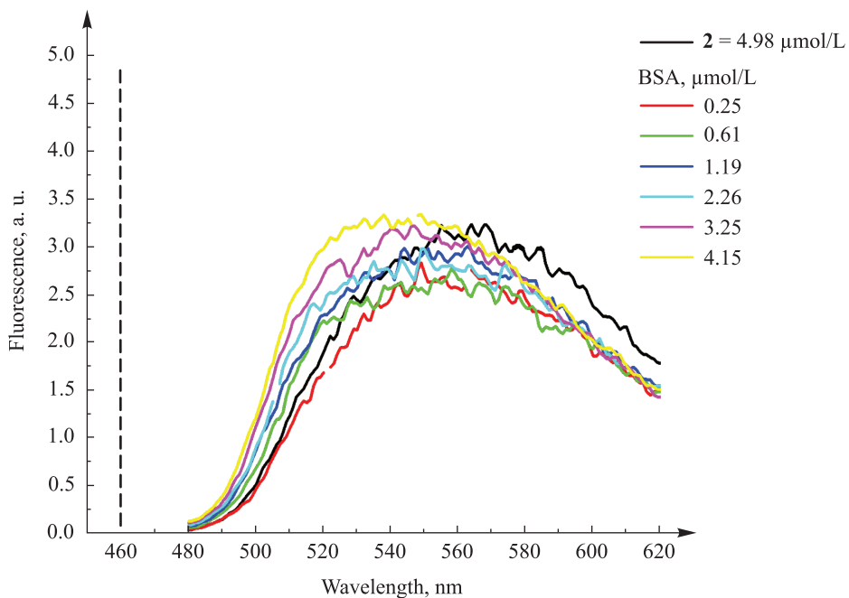
Fig. 6. Fluorescence spectra obtained at BSA interaction with 2 : moderate decrease of BSA fluorescence (excitation at 295 nm) during titration of the protein with 2 (direct titration) ( a ); negligible increase of 2 fluorescence (excitation at 460 nm) during titration of the compound with BSA (inverse titration) ( b )
