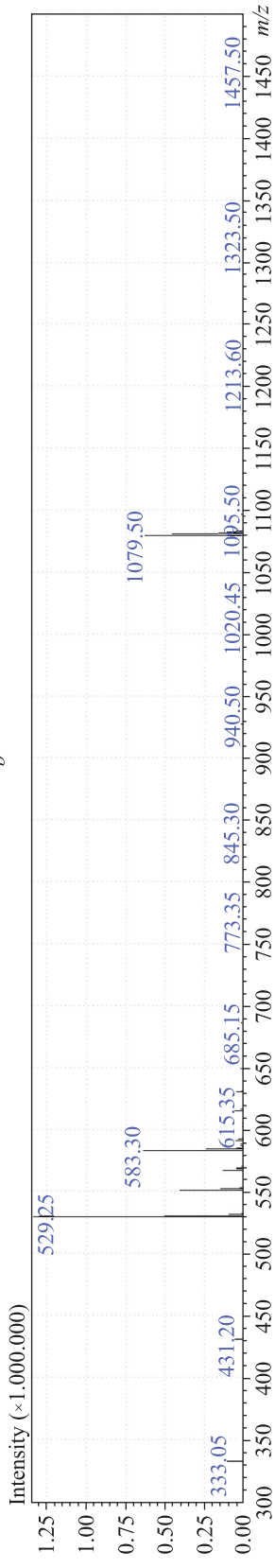
Fig. 3. LC-MS chromatogram (a) and mass-spectrum (b) of FDHex
