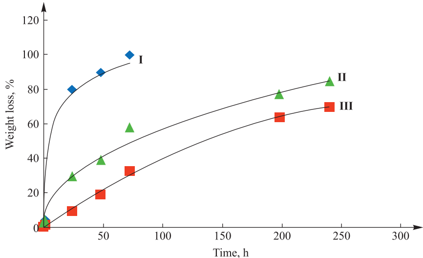
Fig. 4. Weight loss during exposure poly-D,L-lactide (I), poly-D,L- and poly-L-lactide (50 : 50) (II), poly-L-lactide (III) polymer – FDHex composite in 0.1 mol/L NaOH solution
