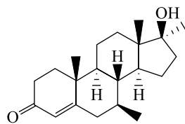
Калустерон (CALS)
