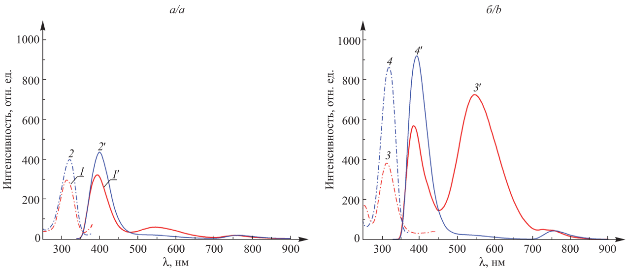
Рис. 3. СВЛ (1, 2) и СЛ (1', 2') образцов № 1 и 2 ( а ); СВЛ (3, 4) и СЛ (3', 4') образцов № 3 и 4 ( б ); \lambda_{\text{ex}} = 320 нм, \lambda_{\text{em}} = 400 нм Fig. 3. Excitation (1, 2) and emission (1', 2') spectra for No. 1 and 2 samples ( a ); excitation (3, 4) and emission (3', 4') spectra for No. 3 and 4 samples ( b ); \lambda_{\text{ex}} = 320 nm, \lambda_{\text{em}} = 400 nm
