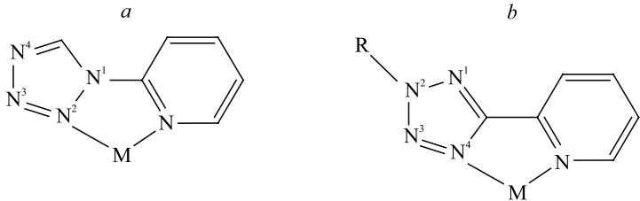
Fig. 2. The structure of the chelate cycle for 2-pytz ( a ) and 2-(2-R-tetrazol-5-yl)pyridines ( b )
