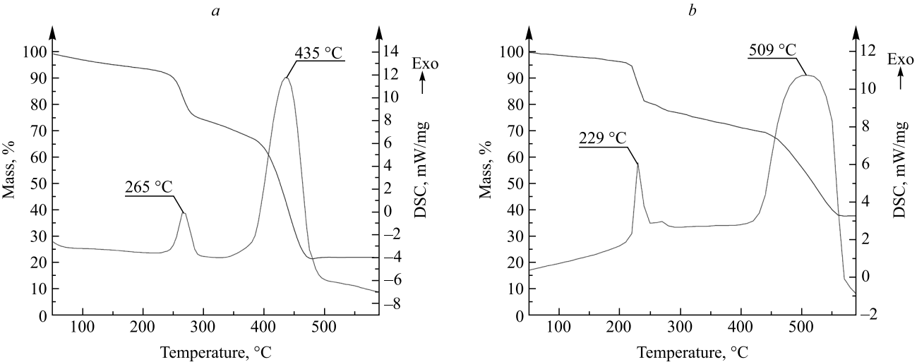
Fig. 5. DSC and TG curves of [Pd(2-pytz)Cl 2 ] (a) and [Pt(2-pytz)Cl 2 ] (b)
