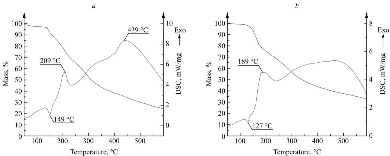
Fig. 6. DSC and TG curves of [Ru(2-pytz)(DMSO) 3 Cl 2 ] · MeOH (a) and [Ru(2-pytz)(DMSO) 2 Cl 2 ] (b)
