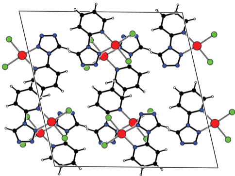
Fig. 9. Crystal structure of [\text{Pd}(\text{2-pytz})\text{Cl}_2] viewed along b axis
