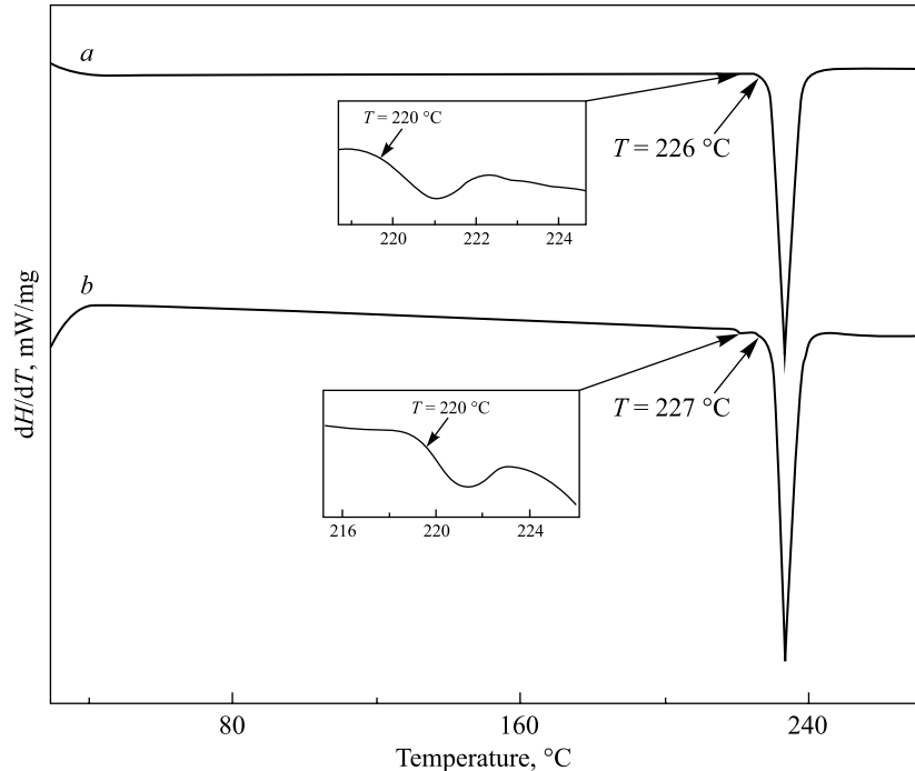
Fig. 2. Differential scanning calorimetry curve for \text{Sn}_{94.7}\text{Ag}_{5.3} (a) and \text{Sn}_{94.0}\text{Ag}_{5.8}\text{Cu}_{1.2} (b) alloys
