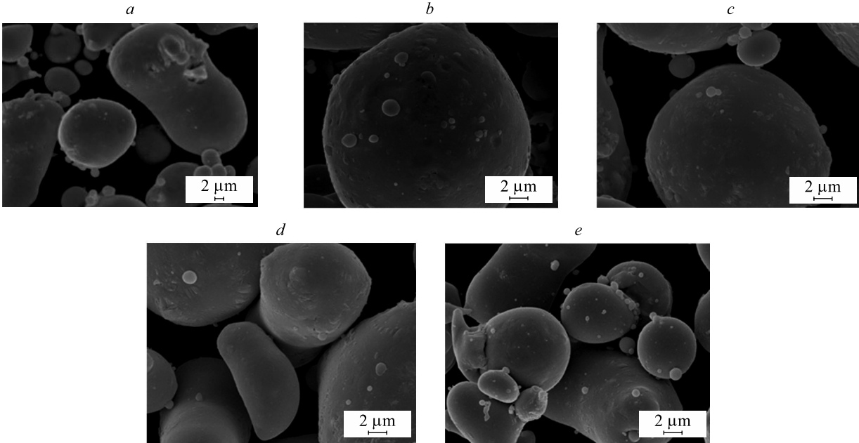
Fig. 3. SEM images of powders: a – Sn; b , e – \text{Sn}_{94.7}\text{Ag}_{5.3} ; c – \text{Sn}_{94.0}\text{Ag}_{4.8}\text{Cu}_{1.2} ; d – \text{Sn}_{99.5}\text{Cu}_{0.5} . Duration of tin powder treatment in pyrophosphate solutions: a – 2 min; b – 15 min; c , d , e – 20 min
