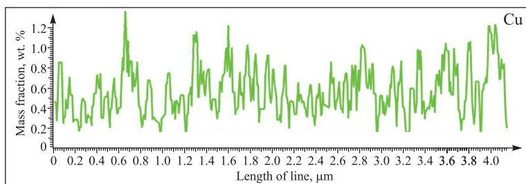
Fig. 4. Local elemental analysis of alloys along the scanning line:
