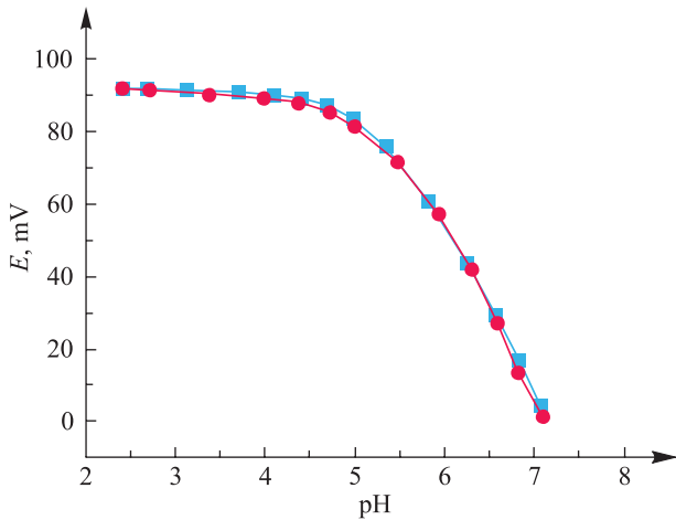
Fig. 4. Dependence of Vin-SE potential on pH
