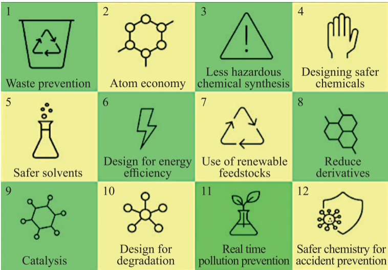
Fig. 5. Principles of green chemistry.
