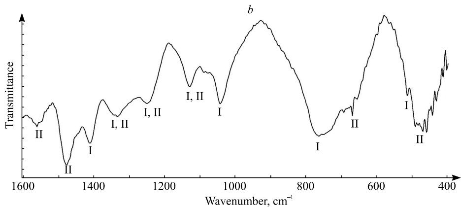
Fig. 5. Calculated IR-spectrum for model E (see fig. 4) (a); experimental IR-spectrum of copper(II) poly-5-vinyltetrazolate (b)
