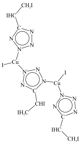
Fig. 3. Supposed copper(II) poly-5-vinyltetrazolate structure (A) and model structures used for calculations (B and C)
