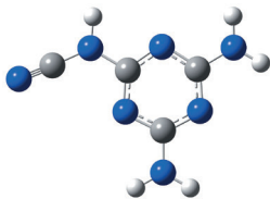
Fig. 7. B3LYP/6-311+G(d, p), Def2-TZVPD optimized model structures of possible products of the poly-5-vinyltetrazole thermolysis
