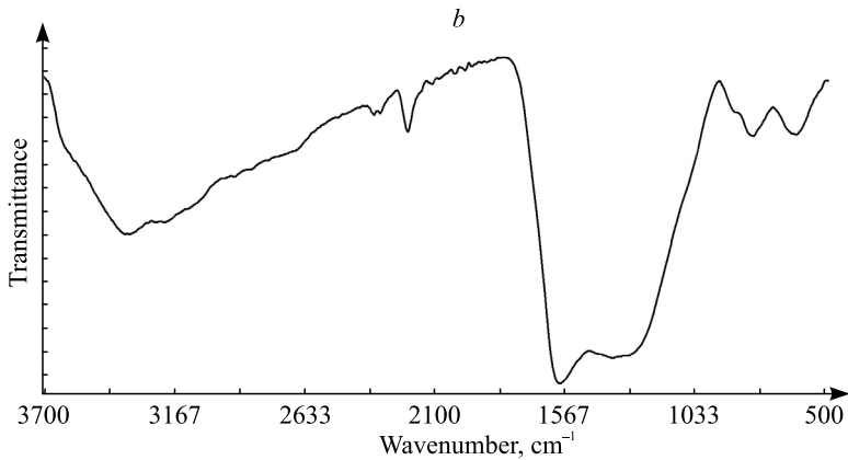
Fig. 8. Calculated IR-spectrum for structure 1 (see fig. 7) ( a ) and experimental IR-spectrum of the product of thermolysis of poly-5-vinyltetrazole ( b )
