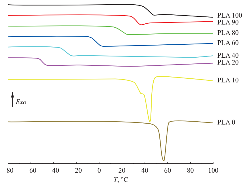
Fig. 2. DCS curves of polylactide (PLA 100), polycaprolactone (PLA 0) and copolymers of D,L-lactide with \epsilon -caprolactone with different content of lactide in the copolymer (PLA 10, PLA 20, PLA 40, PLA 60, PLA 80, PLA 90)
