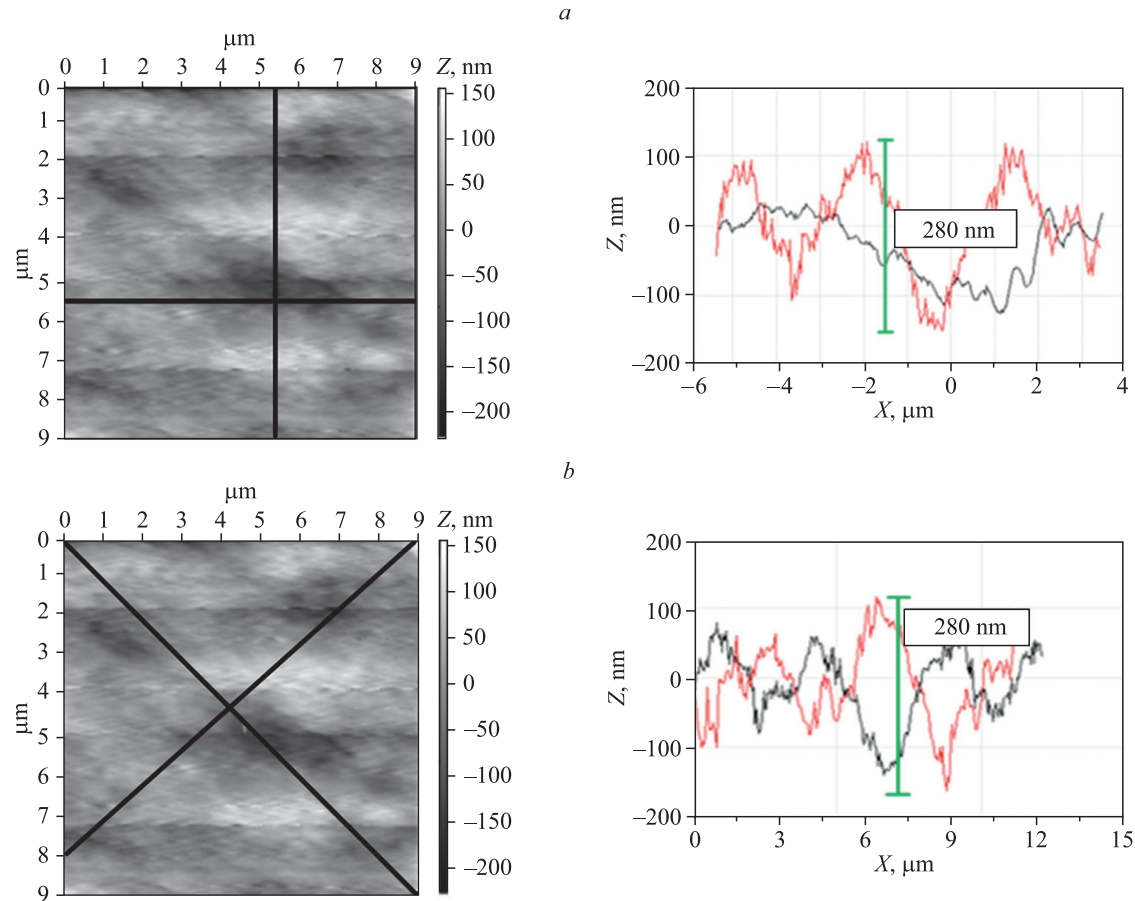
Fig. 1. AFM images and surface relief profiles of as-prepared \text{V}_2\text{O}_5 : \text{MoO}_3 films. The profiles were obtained in the normal directions ( a ) and in the diagonal directions ( b )
