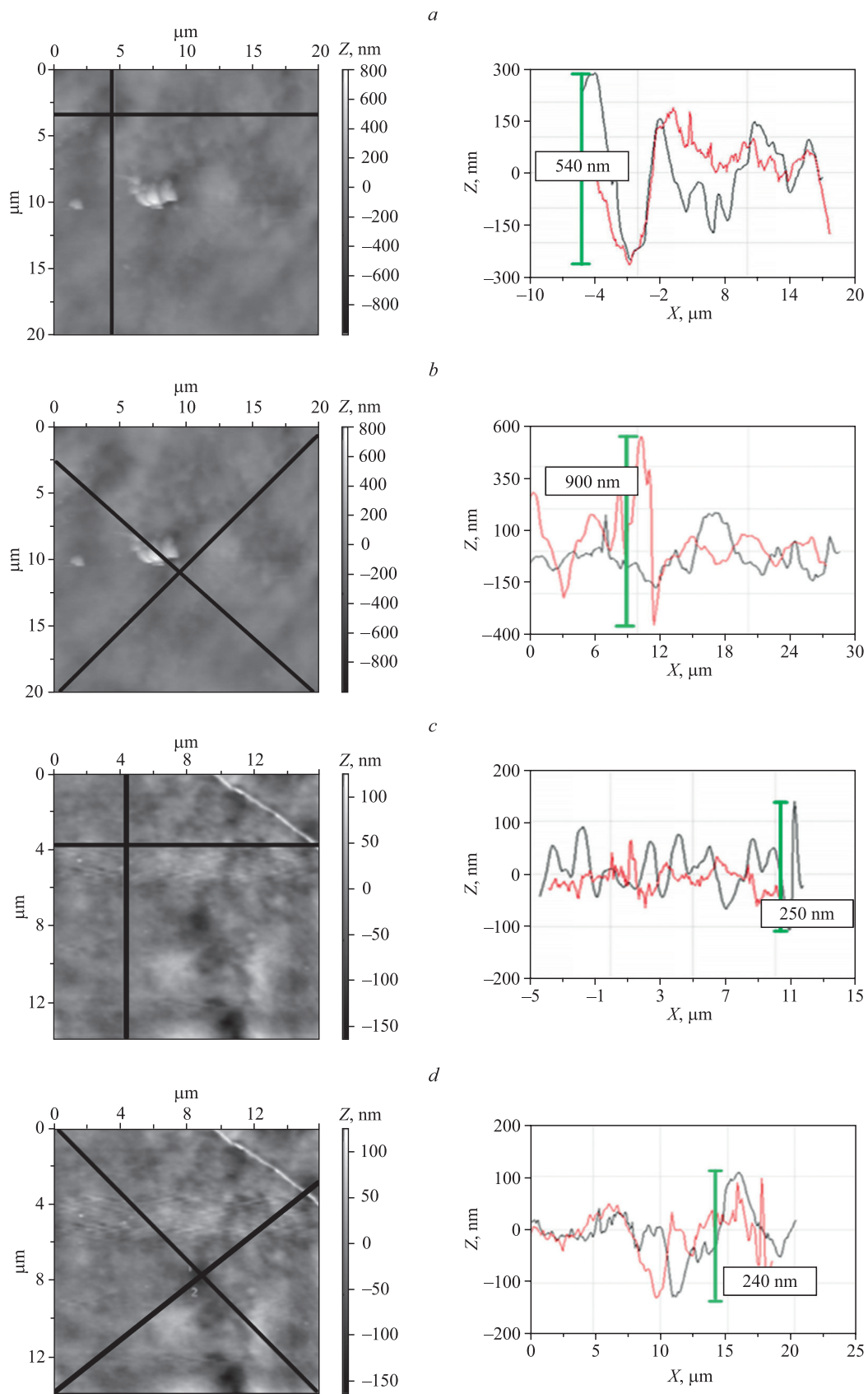
Fig. 2. AFM images and surface relief profiles of \text{V}_2\text{O}_5 : \text{MoO}_3 films exposed to UV-light (a, b) and exposed to UV-light and etched in acid solution for 6 min (c, d). The profiles were obtained in the normal directions (a, c) and in the diagonal directions (b, d)
