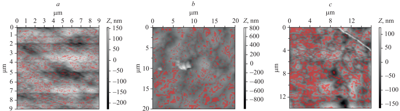
Fig. 5. Faceted structures (shown in red) forming nuclei at the surface of \text{V}_2\text{O}_5 : \text{MoO}_3 films: a – as-prepared film; b – the film exposed to UV-light; c – the film exposed to UV-light and etched in acid solution for 6 min
