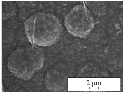
Fig. 3. SEM images of the surface of nickel ( a ) and \text{Ni} - 0.6\text{MoO}_3 : 0.4\text{V}_2\text{O}_5 ( b )
