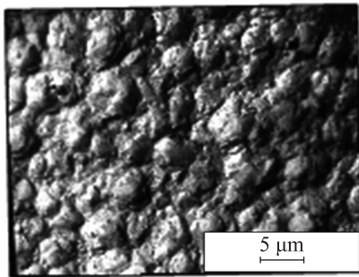
Fig. 3. SEM images of the surface of nickel ( a ) and \text{Ni} - 0.6\text{MoO}_3 : 0.4\text{V}_2\text{O}_5 ( b )
