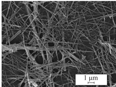
Fig. 2. SEM images of dispersions of x\text{MoO}_3 : (1 - x)\text{V}_2\text{O}_5 oxide particles ( x = 0.25 (a); x = 0.4 (b); x = 0.75 (c))
