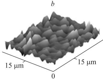
Fig. 4. AFM images of the surface of nickel ( a ) and Ni – 0.6MoO 3 : 0.4V 2 O 5 ( b )
