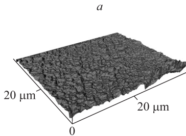
Fig. 4. AFM images of the surface of nickel ( a ) and Ni – 0.6MoO 3 : 0.4V 2 O 5 ( b )
