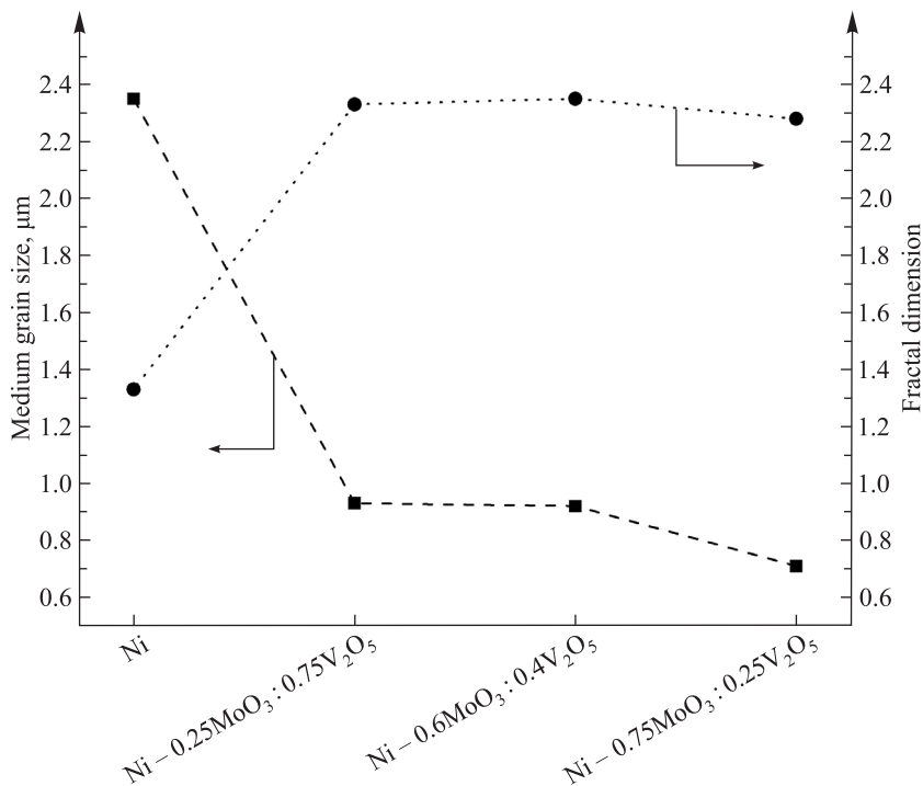
Fig. 5. Dependence of the medium size of nickel grains and fractal dimension of a surface for galvanic nickel and \text{Ni} - x\text{MoO}_3 : (1 - x)\text{V}_2\text{O}_5 composite films of different composition
