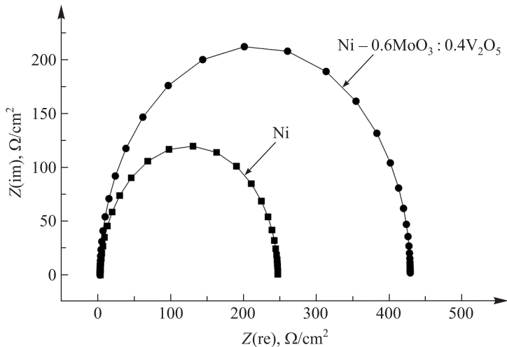
Fig. 7. Electrochemical impedance spectra of bare galvanic nickel and \text{Ni} - 0.6\text{MoO}_3 : 0.4\text{V}_2\text{O}_5 composite in 0.5 mol/L NaCl aqueous solution used as the corrosion medium. Measurements were done under open circuit potentials
