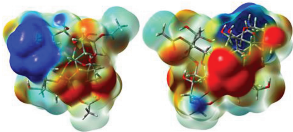
Fig. 17. MEP mapped on an SCF density of complex KAN – CAS
