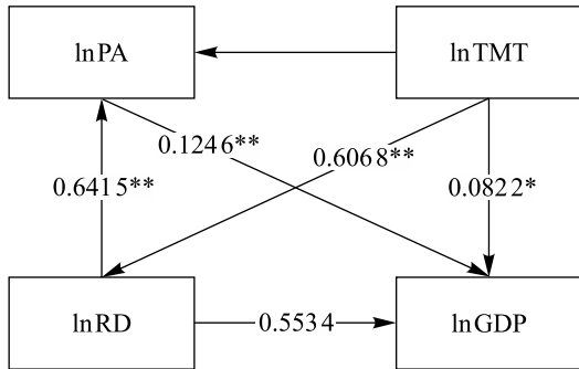
Fig. 5. Static Bayesian network diagram
