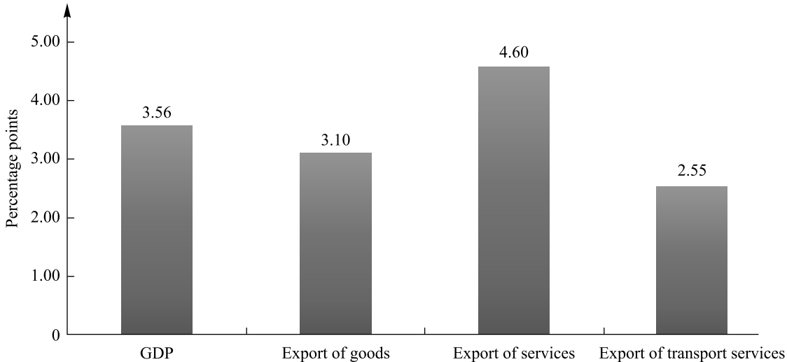
Fig. 1. Average annual growth rates of world GDP, exports of goods, services and transport services after the global financial crisis in 2007–2018. (authors' calculations based on UNCTAD [7] data)
