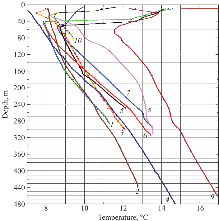
Fig. 4. Selected temperature logs of boreholes in the vicinity of Grodno:
