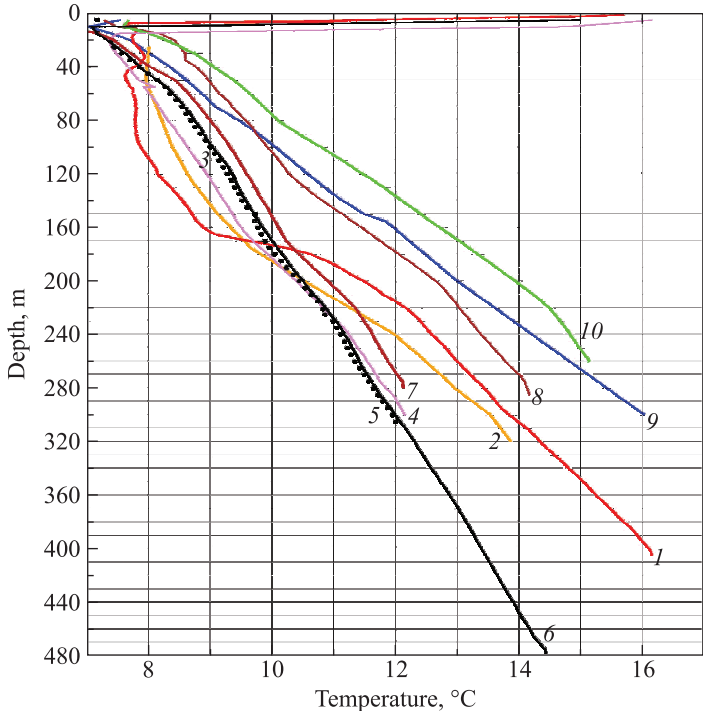
Fig. 5. Selected temperature logs of boreholes in the Privalka and Porechye areas:
