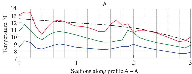
Fig. 10. Temperature distribution along B – B ( a ) and A – A ( b ) profiles of the Grodno region at depths of 100 m (blue line), 200 m (green line), and 300 m (red line)
