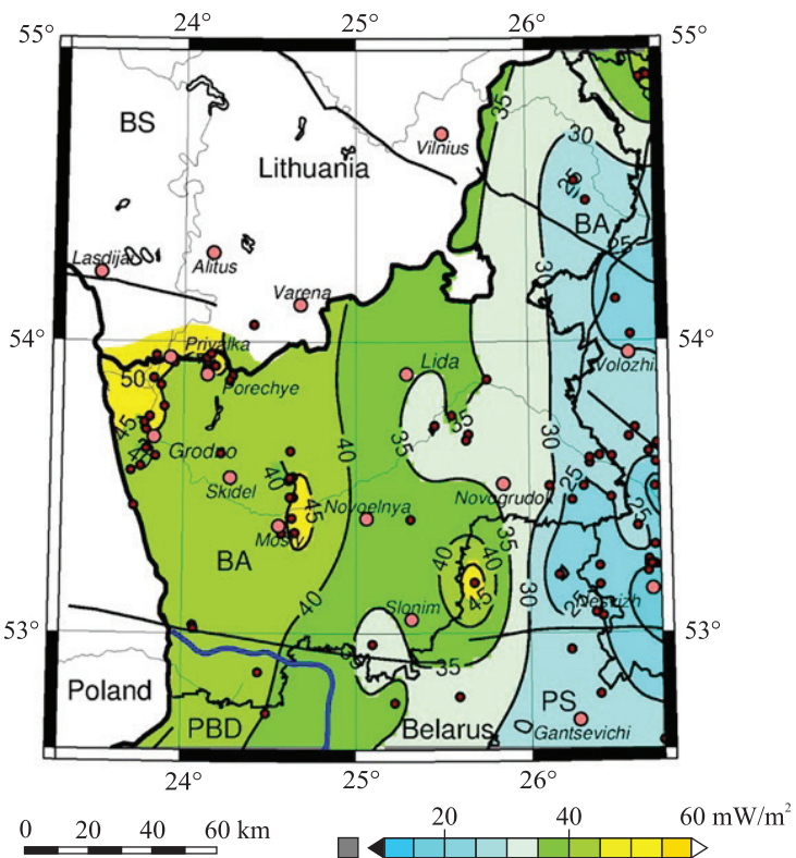
Fig. 11. Heat flow density map
