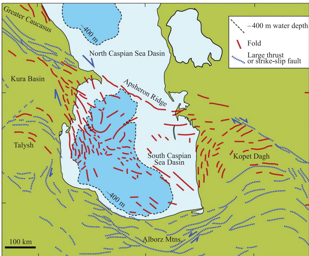
Fig. 2. Main faults and deep-water areas within the Central Caspian and South Caspian Basins, respectively.
