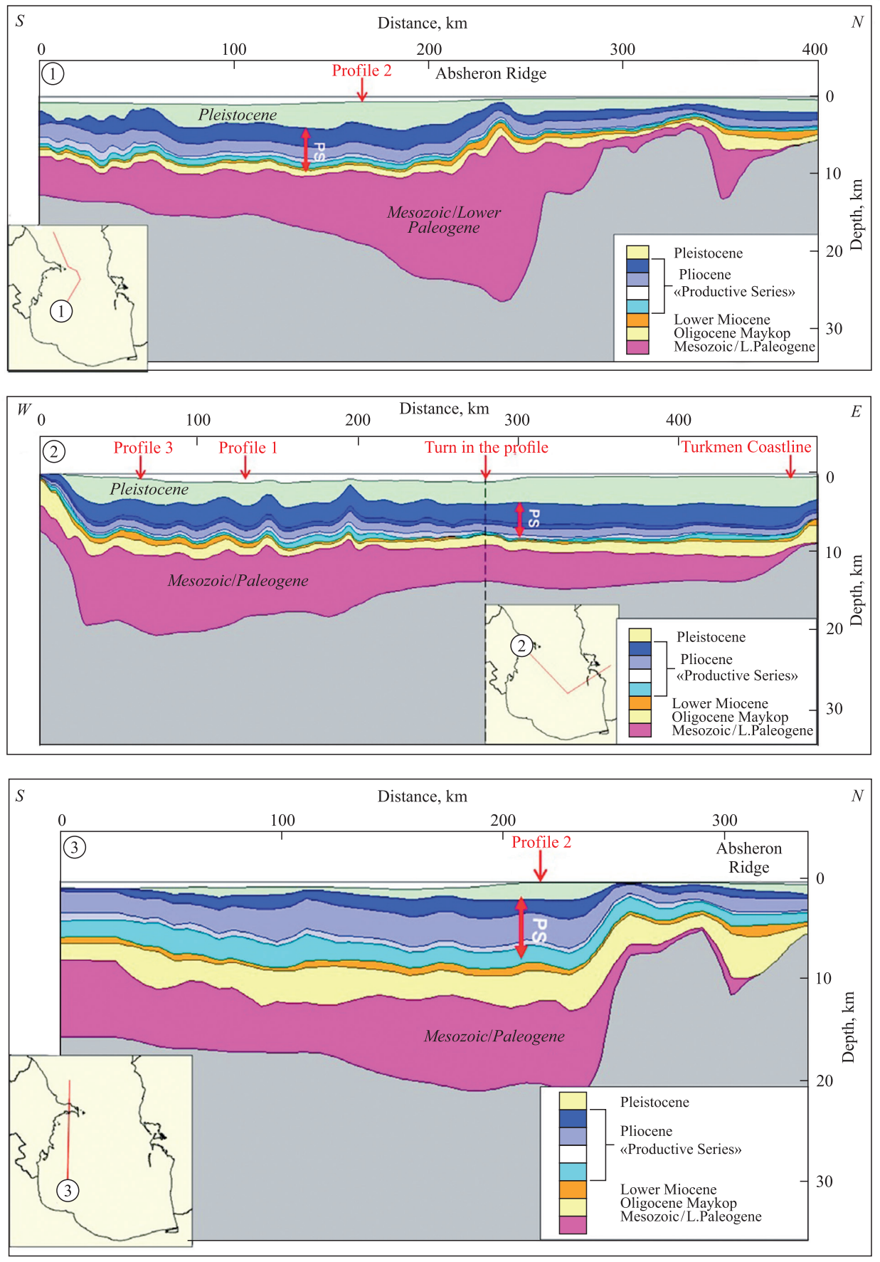
Fig. 3. Seismic profiles through the South Caspian Basin.
