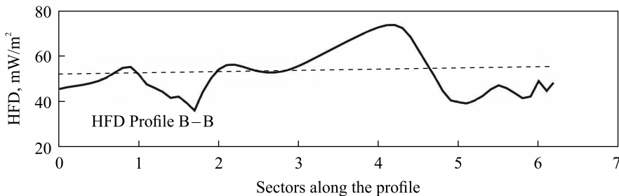
Fig. 11. Heat flow density profiles A-A and B-B
