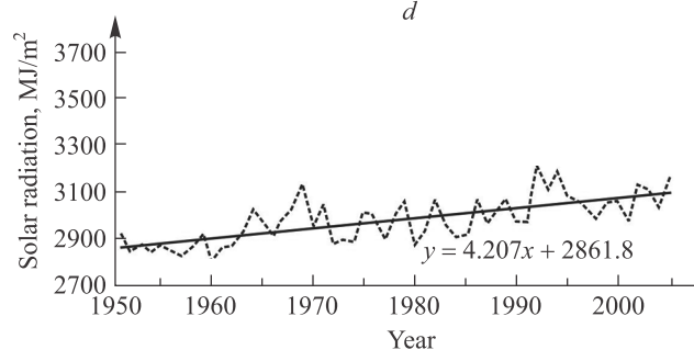
Fig. 3. Multi-annual course of total solar radiation for selected grid points in Central Europe in the period of 1951–2005: a – 54.29° N., 16.88° E.; b – 54.29° N., 20.63° E.; c – 50.48° N., 16.88° E.; d – 50.48° N., 20.63° E.
