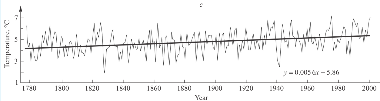
Fig. 2. Course of annual air temperature values and the trend line in Warsaw (a), Vilnius (b) and Tallinn (c).
