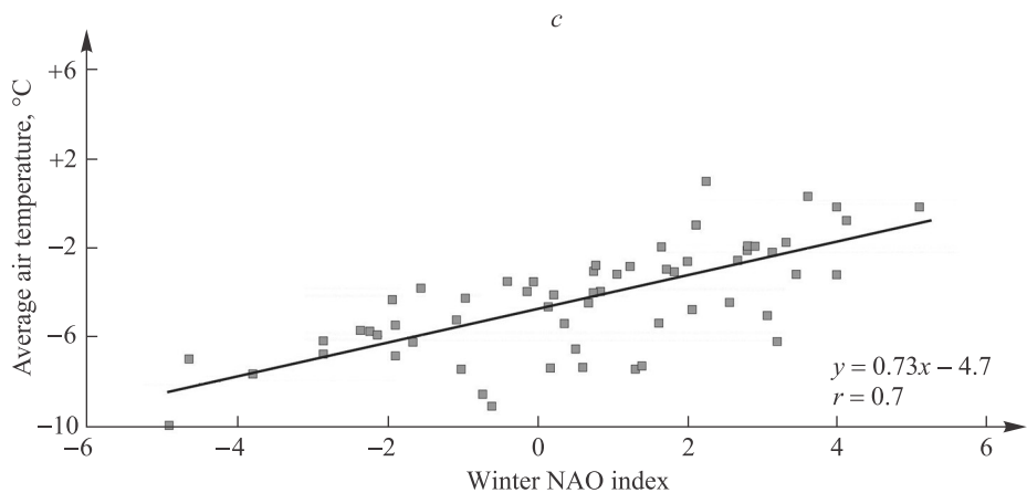
Fig. 5. The relationship between the average air temperature in December – March and the winter NAO index (DJFM) in the period of 1971–2020 for the stations Gorzow ( a ), Olsztyn ( b ), Vitebsk ( c )
